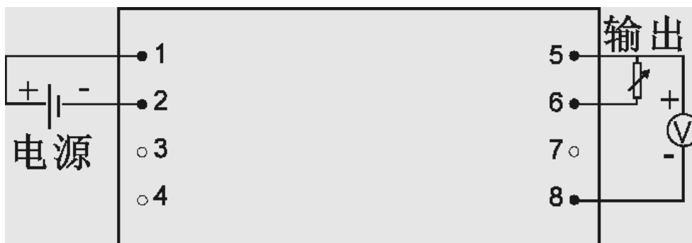
GRBxxxxD-xW-B B Model Connection Diagram (bottom view)
